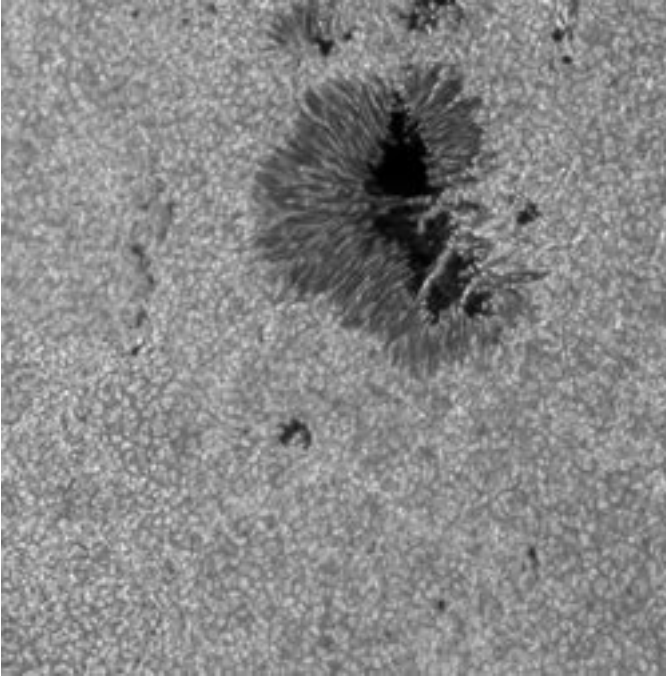
Fig. 2: A large sunspot visible on the Sun in June 2000. The picture shows a section of the Sun's surface 80,000 by 80,000 km across. Sunspots appear darker than their surroundings because their strong magnetic fields suppress the energy transported by gas flows. This picture was taken with the German Vacuum Tower Telescope at the Observatorio del Teide (Teneriffe).
