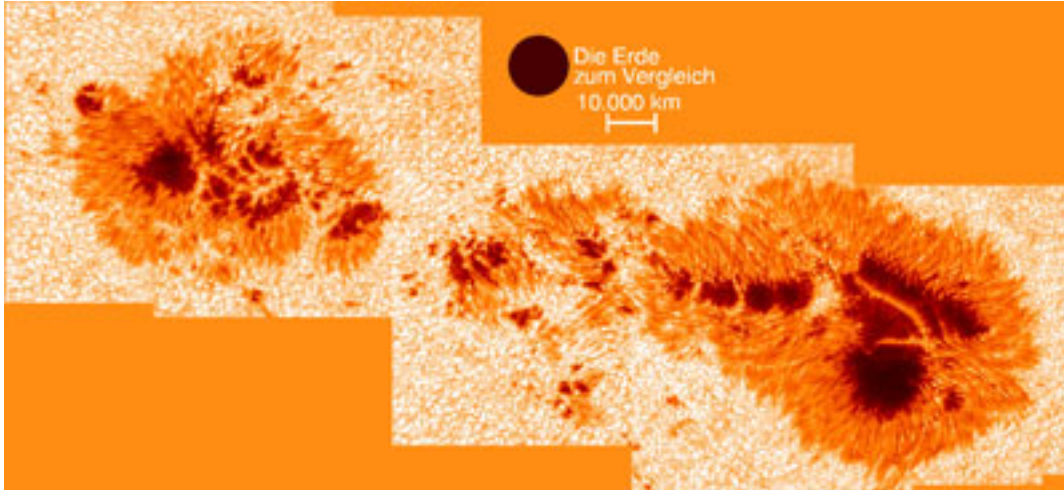
Fig. 1: Extended group of sunspots visible in the southern hemisphere of the Sun in September 1998. These sunspots are fascinating not only due to their large size, but also due to their detailed structure that reveals a dynamic complexity. The smallest visible features are about 350 km across, the entire area covers about 200,000 km in the horizontal direction. The sub-pictures in this mosaic were obtained with the German Vacuum Tower Telescope at the Observatorio del Teide (Teneriffe).
